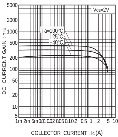
Fig.4 DC current gain vs. collector current
