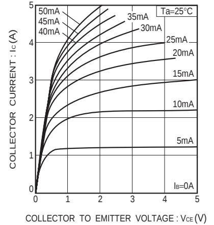
Fig.3 Grounded emitter output characteristics (II)
