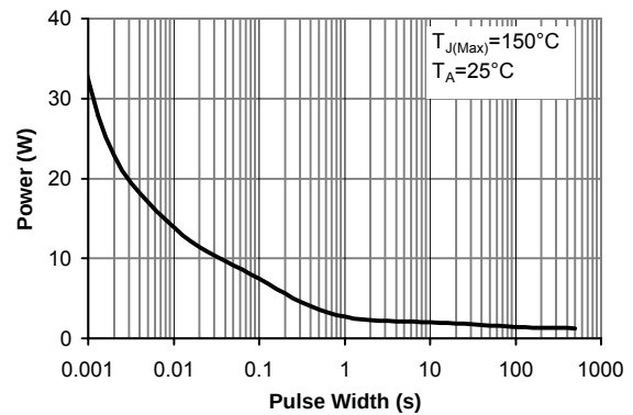
Figure 10: Single Pulse Power Rating Junction-to-Ambient
