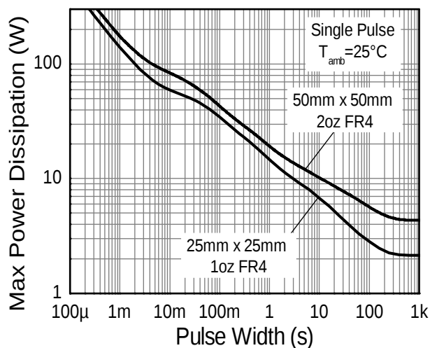
Pulse Power Dissipation
