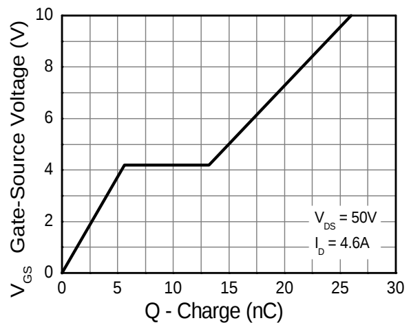
Gate-Source Voltage v Gate Charge
