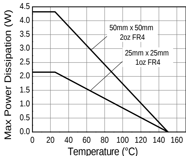
Derating Curve
