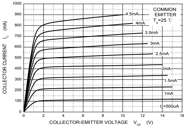
Static Characteristic
