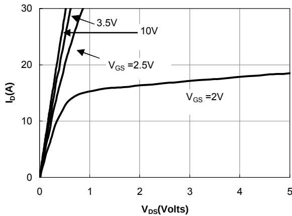
Figure 1: On-Regions Characteristic
