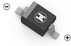
SOD-323
