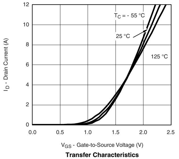
Transfer Characteristics
