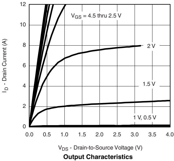
Output Characteristics
