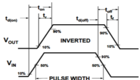
Figure8. Switching wave
