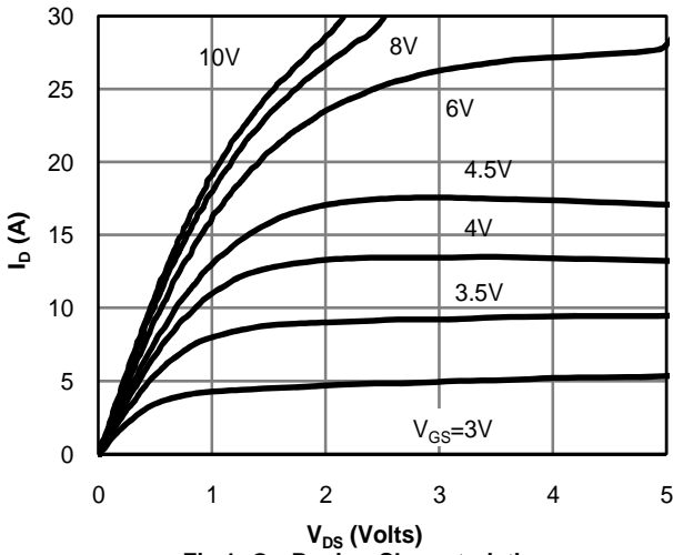
Fig 1: On-Region Characteristics
