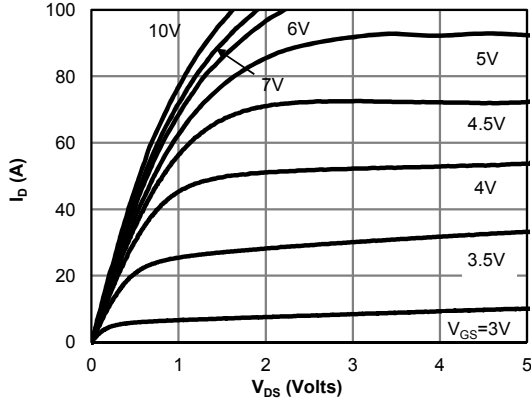
Fig 1: On-Region Characteristics
