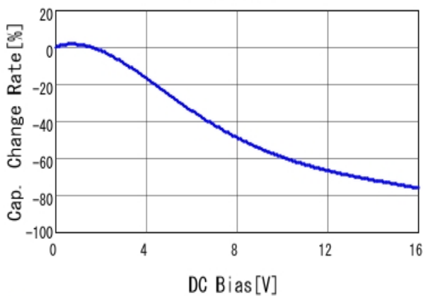
■ GRM188R71C105ME15 C-DC bias capchange, 25.0degC, AC1V
