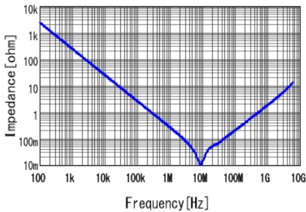
■ GRM188R71C105ME15 |Z| DCOV, 25degC
