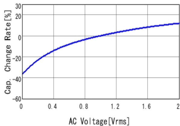
■ GRM188R71C105ME15 C-AC Voltage capchange, DCOV, 25.0d
